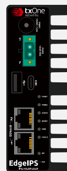
Front Panel
